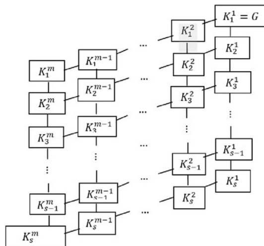
Figure 1: Rectangle Lattice
